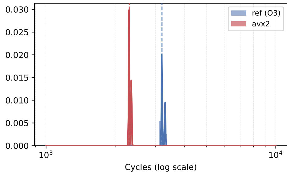
noise \eta_1 ( \sim 1.3\times speedup)
