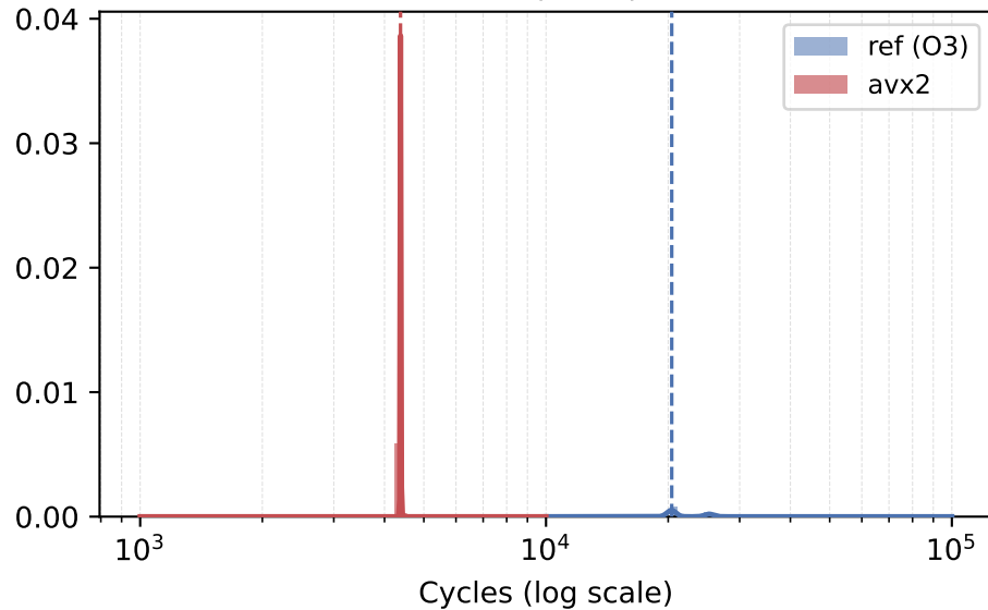
gen_a ( \sim 4\times speedup)
