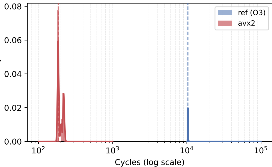
INVNTT ( \sim 55\times speedup)
