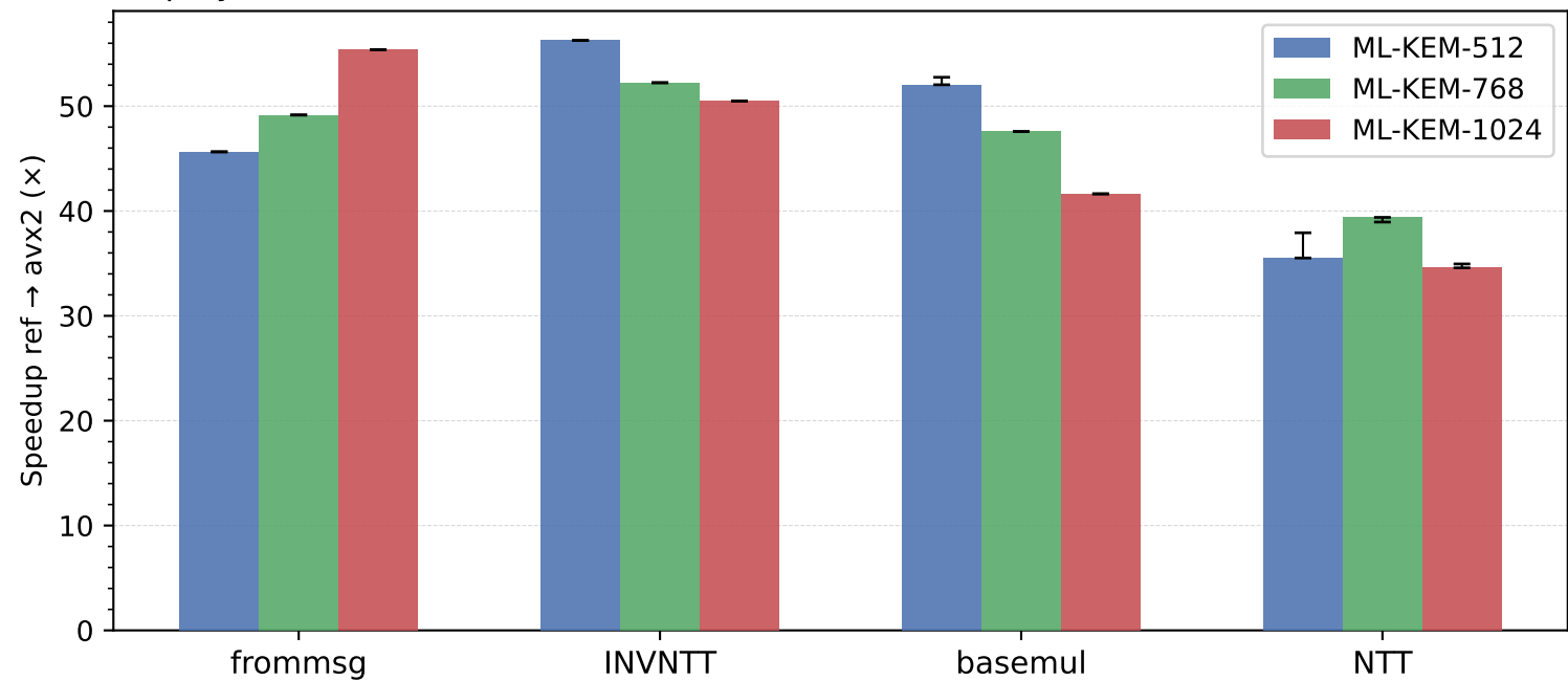
Per-Polynomial Operation Speedup Across Security Parameters (polynomial dim = 256 for all; NTT variation attributed to cache-state differences)
