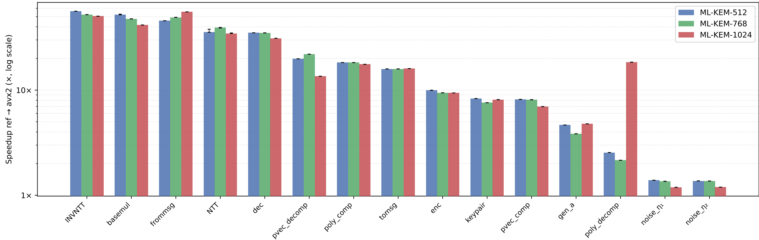
Hand-Written SIMD Speedup over Compiler-Optimised C (Intel Xeon Platinum 8268, 95% bootstrap CI, n≥2000 per group)
