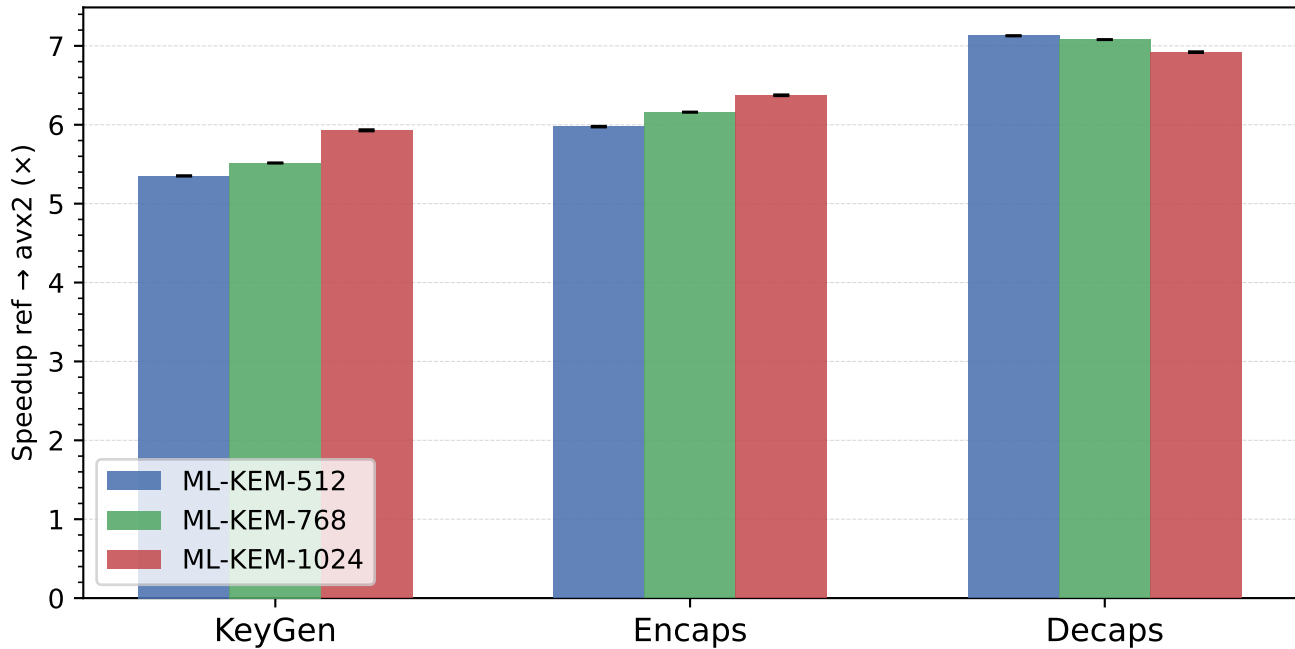
End-to-End KEM Speedup (ref \rightarrow avx2) (Intel Xeon Platinum 8268, 95% bootstrap CI)
